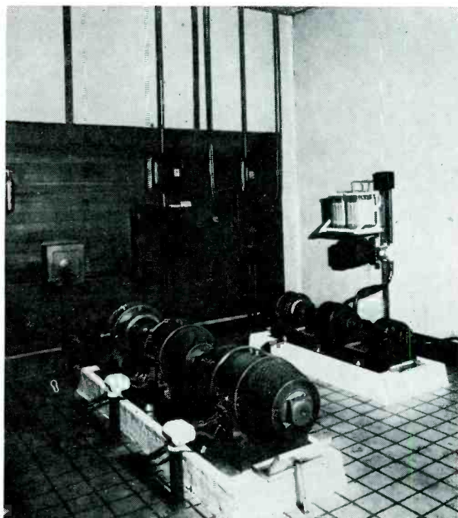
Fig. 2. Generator room at an early station. The large motor-generator supplied plate power, the other powered the filaments.
