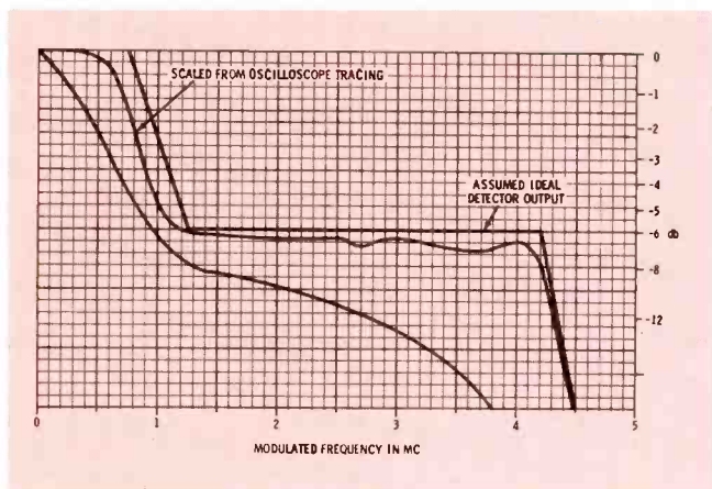
Fig. 3. Video response is shown by tracing of scope display.
