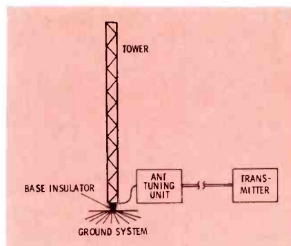
Fig. 5. A simple equipment arrangement like this is sufficient for a site test.
