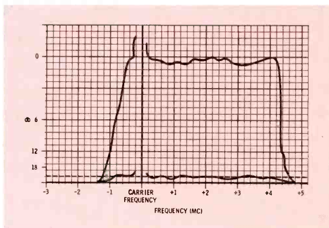
Fig. 4. Attenuation vs frequency is shown by display tracings.
