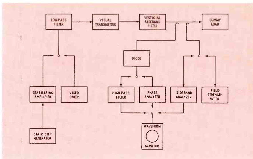
Fig. 2. Diagram similar to this can be used to show setups for tests on video transmitter.
